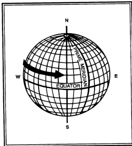
Figure 7-1. Rotation of the earth
